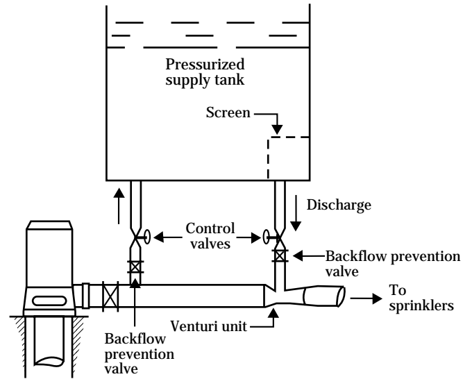
Figure 7-5 Venturi principle of injection
